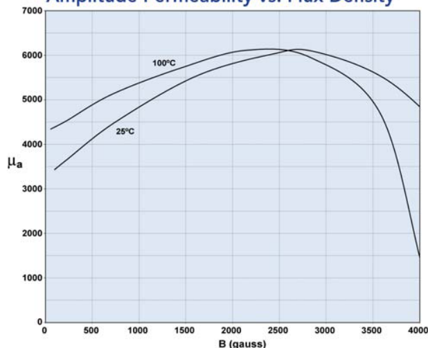
Amplitude Permeability vs. Flux Density
